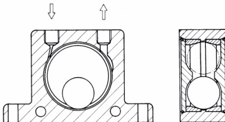
Housing made from extruded aluminium alloy Hardened guides made of steel Nylon end plates Hardened ball
